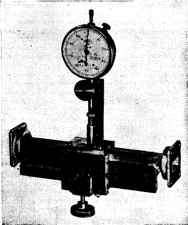
FIG. 18-10.—Adjustable transformer.
